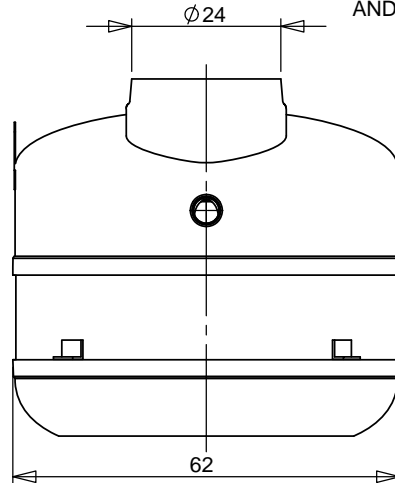
EXTENSION COLLAR SEAT DETAIL "A" LABEL INSIDE AND OUT
