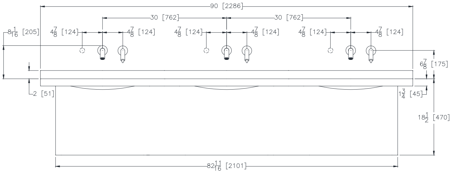
FRONT VIEW
