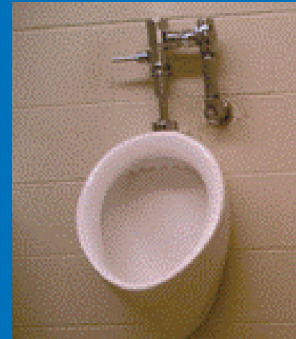
University of Washington: Non-Zurn 0.5 GPF urinal system. Notice the alter- ations made in the piping in order to fit the footprint.
