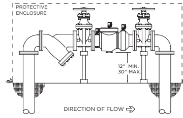
OUTDOOR INSTALLATION
