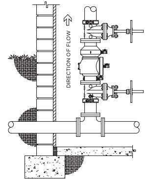
VERTICAL INSTALLATION (3500SY)
