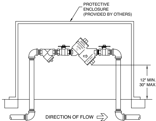
OUTDOOR INSTALLATION
