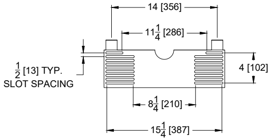
UNIVERSAL RETROFIT BRACKET (UB)
