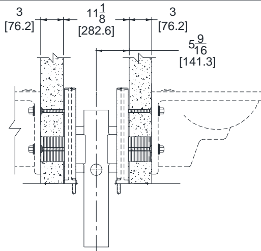
Z1209-ND4 DOUBLE IN BLOCK WALL
