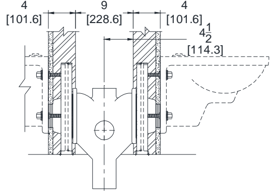
Z1204-ND4 DOUBLE IN METAL STUD WALL
