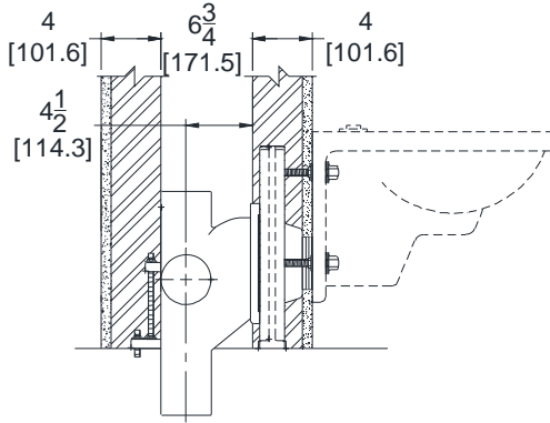
Z1204-N4 SINGLE IN METAL STUD WALL
