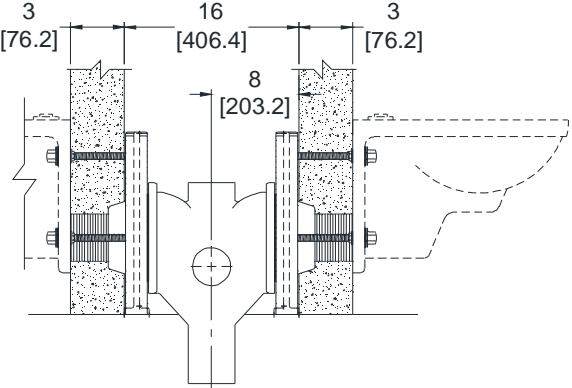
Z1204-ND4 DOUBLE IN BLOCK WALL
