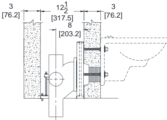
Z1204-N4 SINGLE IN BLOCK WALL
