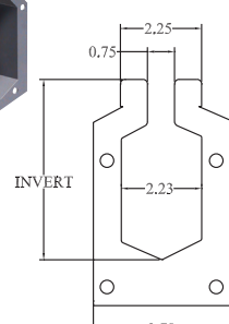
Z891 5' Length; Pre-Sloped, Stainless Steel
