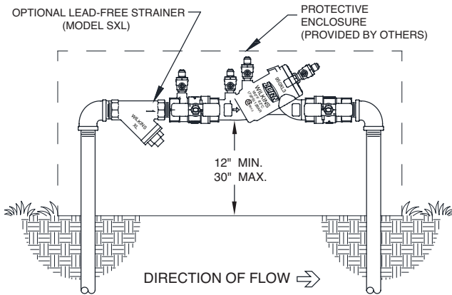
OUTDOOR INSTALLATION
