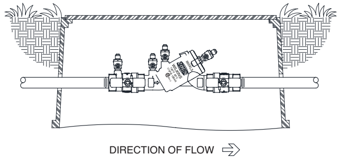
PIT INSTALLATION
